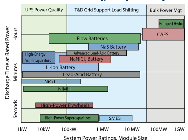
Characteristics of Energy Storage Technologies 12
