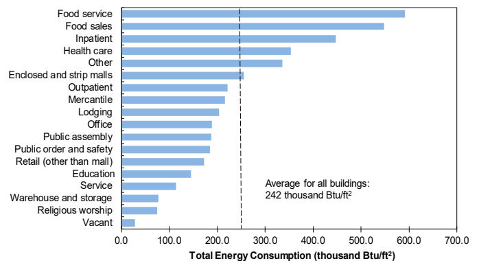
Total Energy Consumption, U.S. Commercial Buildings, 2012 13
