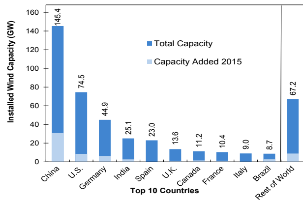
Global Wind Capacity, 2015 15
