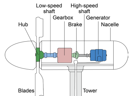
Horizontal Axis Wind Turbine Diagram 9,12
