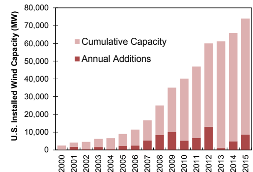
U.S. Wind Capacity 13,14
