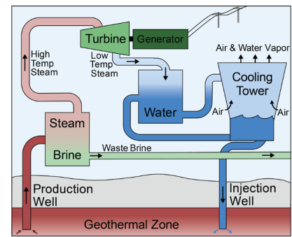
Flash Steam Geothermal Power Plant 14
