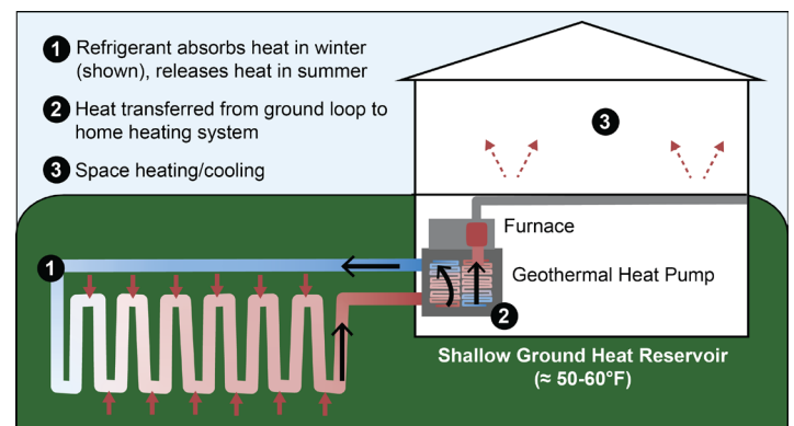
Geothermal Heat Pump in a Residential Heating Application 9
