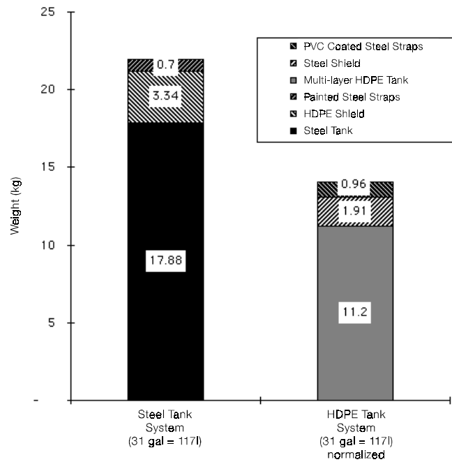
Fig. 1: Composition of fuel tank systems
