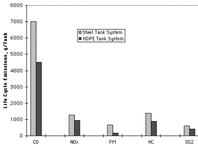
Fig. 6: Cumulative life cycle air emissions
