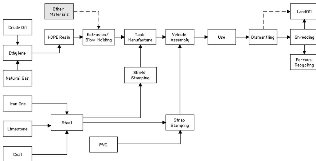
Fig. 3: HDPE fuel tank system
