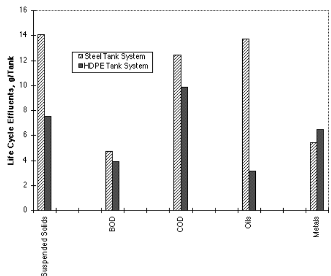
Fig. 7: Cumulative life cycle water emissions
